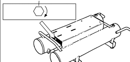
Figure 4 Clockwise rotation of 1/2" bolt will increase belt tension
