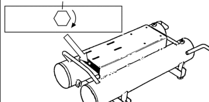
Figure 4 Clockwise rotation of 1/2" bolt will increase belt tension
